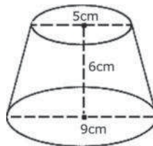
Cone dimensions
